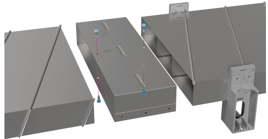
INSTALLATION VIEW
